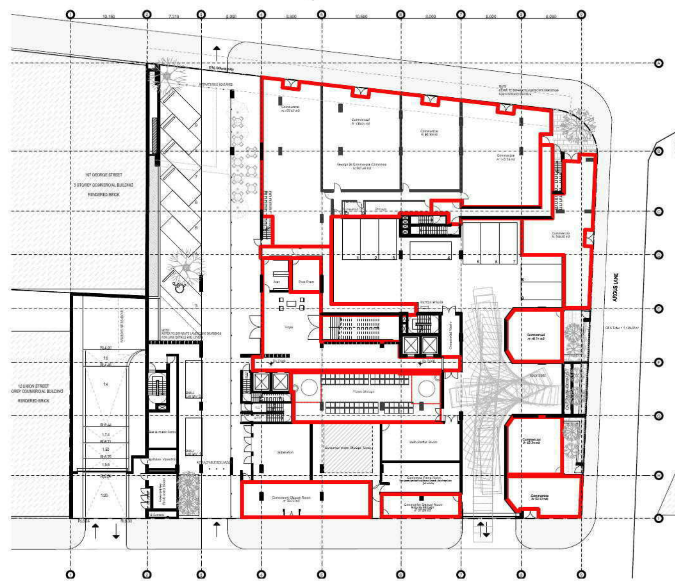
6 GFA Ground Floor Level 01 1:500
